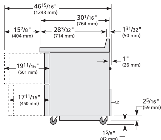
RIGHT VIEW
